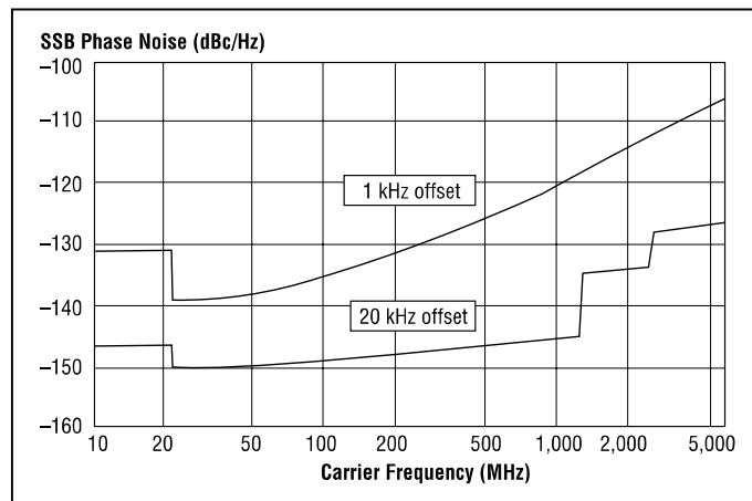
Typical Phase Noise Variation with Frequency
